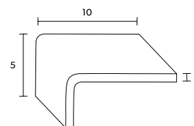
CANTONEIRA 10X5
